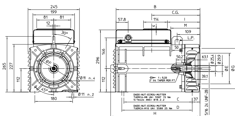
FORMA - FORM J609b
