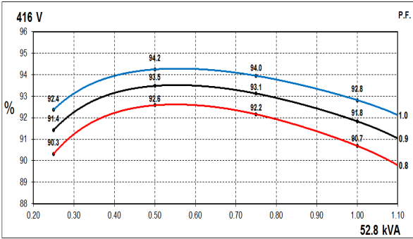
60Hz Curves
