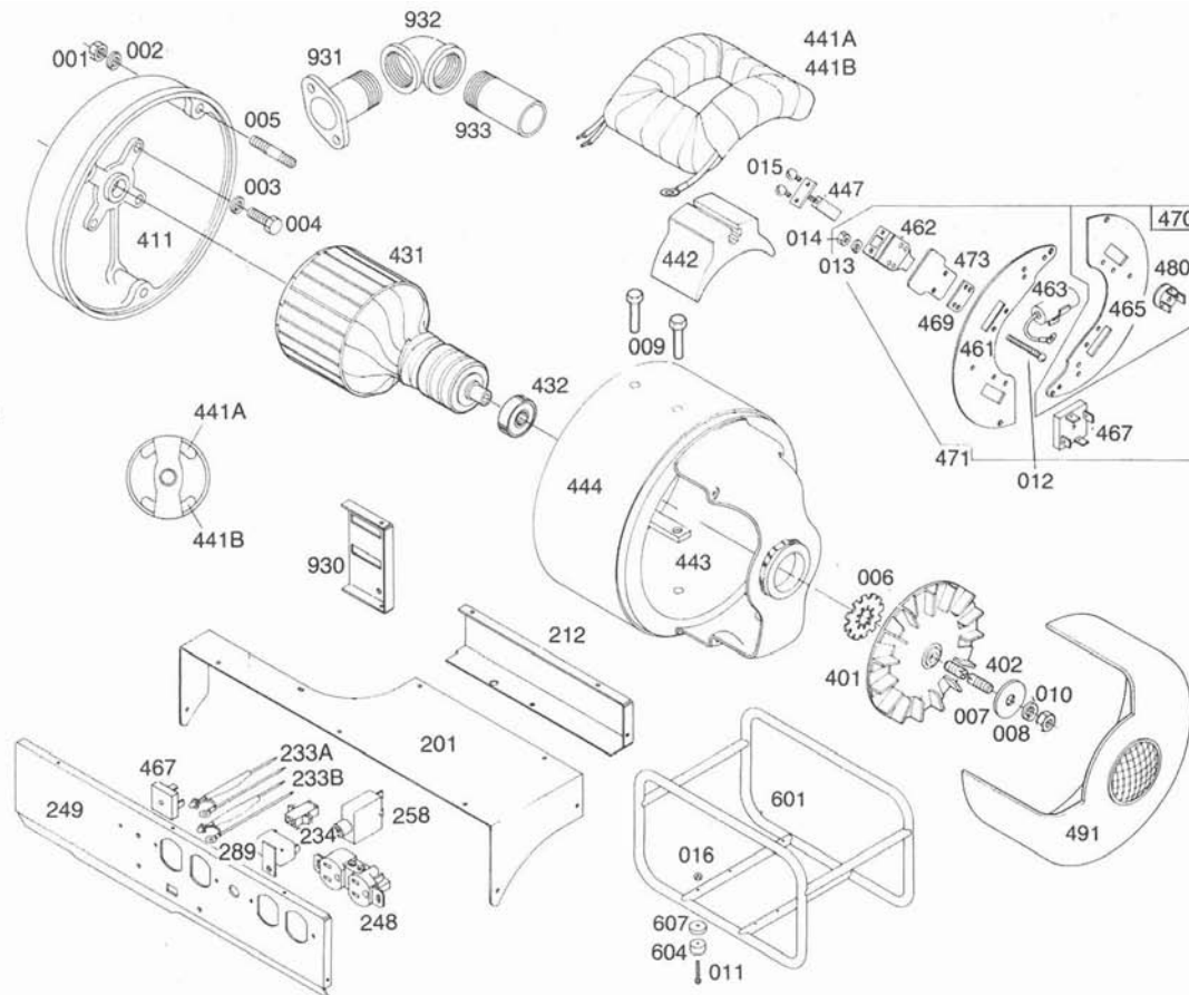
Figure 2 — Replacement Parts Illustration
