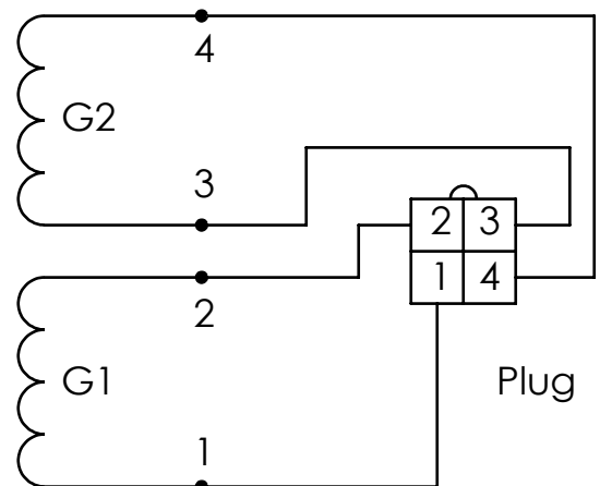
Power Winding
