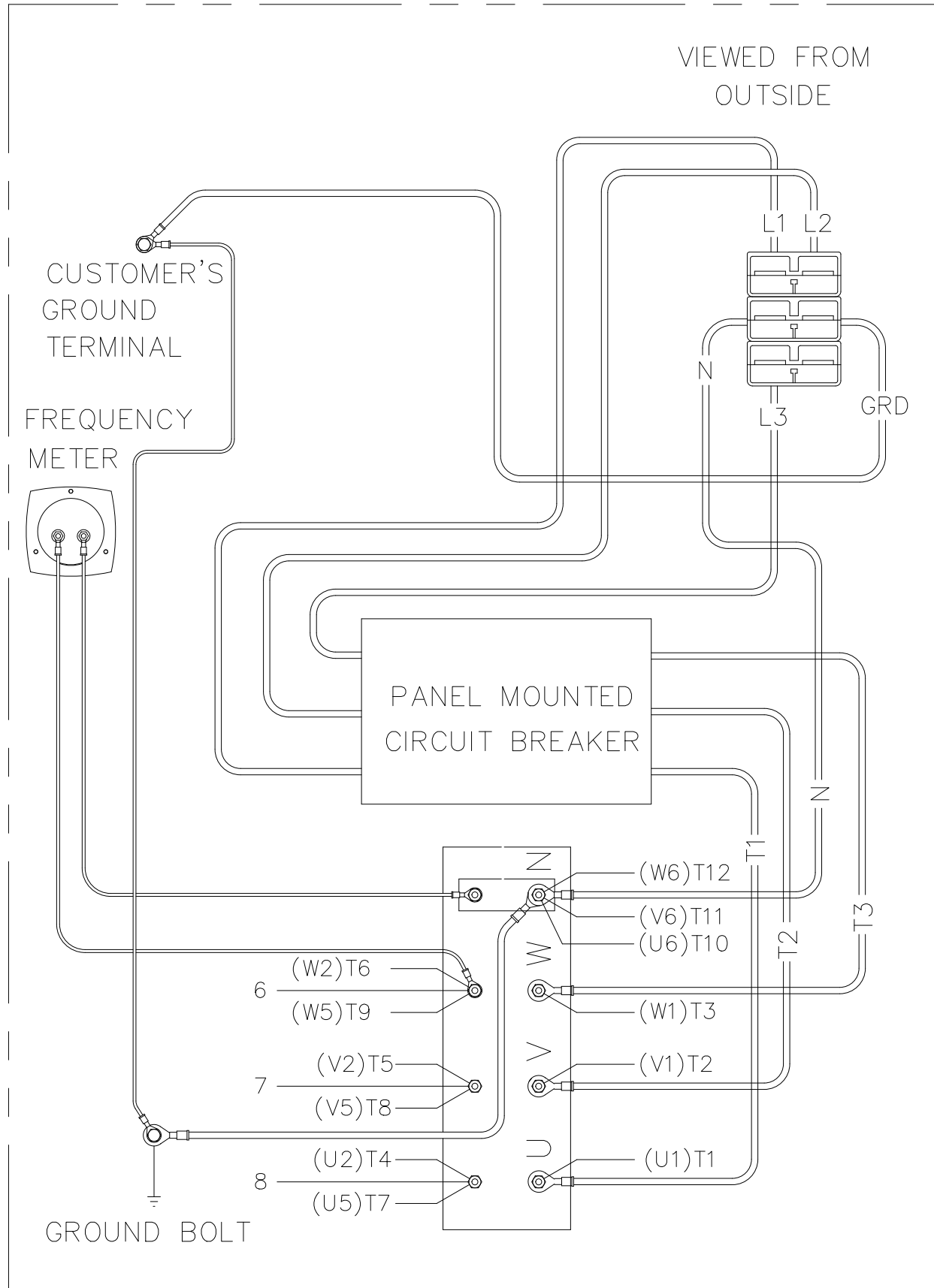
WIRING DIAGRAM (THREE PHASE WYE "12 WIRE"; 277/480)
