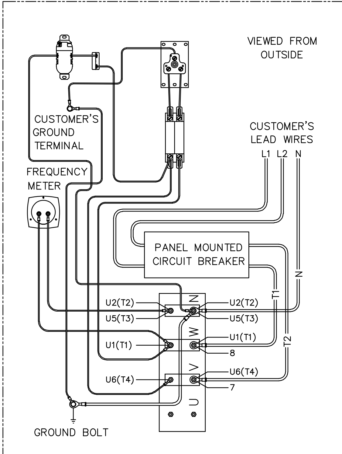
WIRING DIAGRAM (SINGLE PHASE "4 WIRE"; 120/240)
