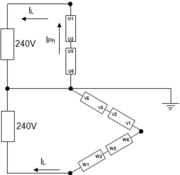
Zig Zag 2 - 240V 60Hz
