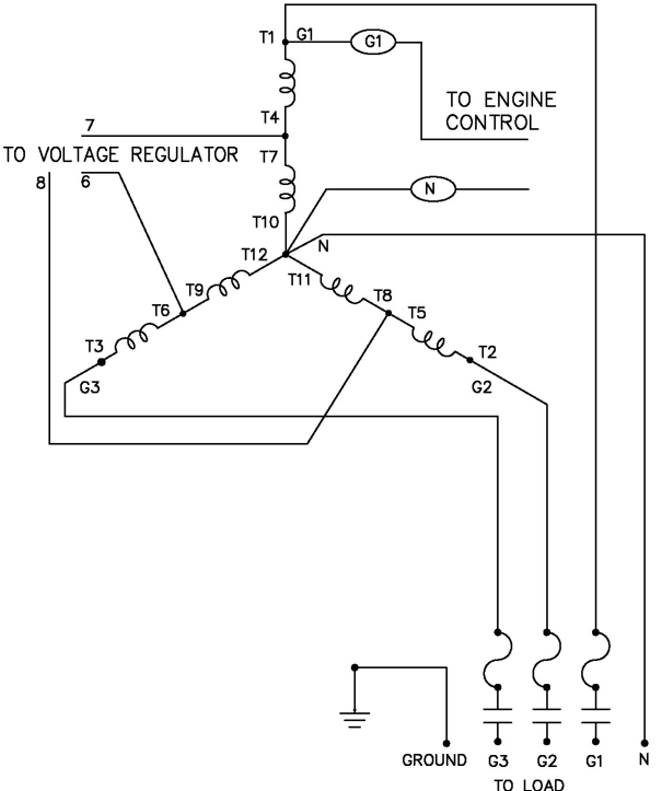
High Voltage Wye 240/416 - 277/480V 60Hz
