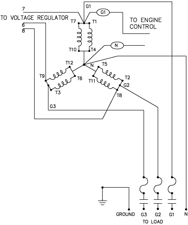
Low Voltage Wye 120/208V 60Hz
