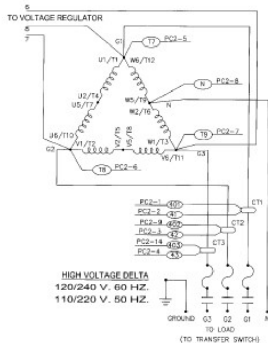
THREE PHASE DELTA 120/240V
