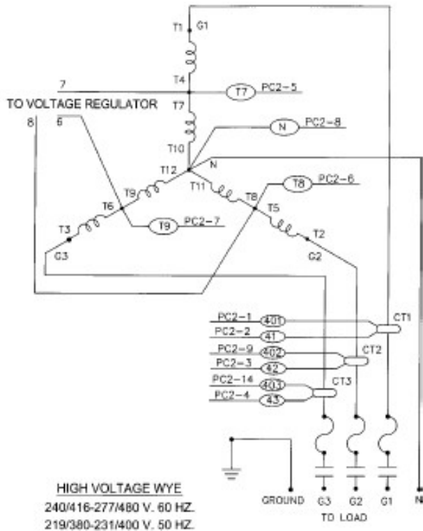
THREE PHASE - HIGH WYE 277/480V
