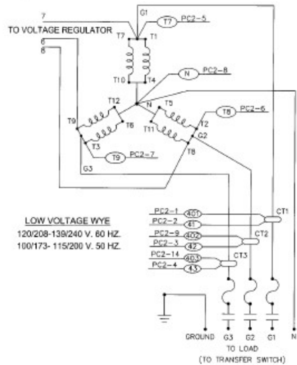
THREE PHASE - LOW WYE 120/208V
