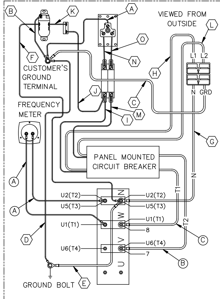
WIRING DIAGRAM (SINGLE PHASE "4 WIRE"; 120/240)
