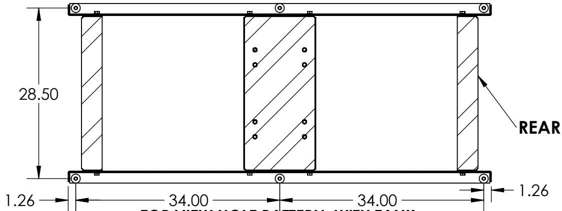
TOP VIEW HOLE PATTERN, WITH TANK
