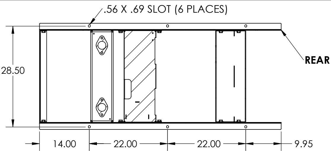
TOP VIEW HOLE PATTERN, NO TANK
