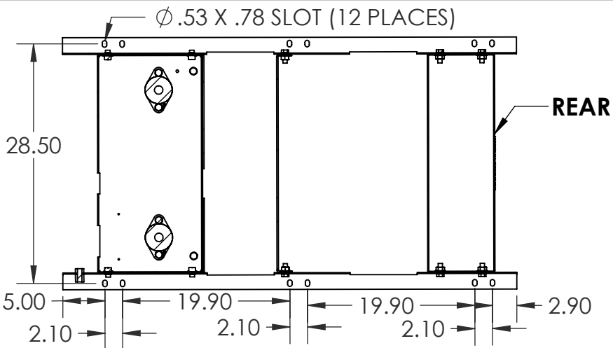
TOP VIEW HOLE PATTERN NO TANK
