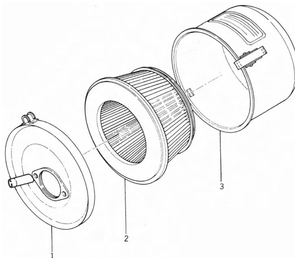
KF150D-SX (316522) Fig. A-1 AIR CLEANER
