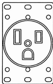
NEMA: 5-50R 125V-50A
