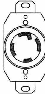
NEMA: L14-30R 125/250V-30A
