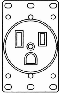
NEMA: 5-50R 125V-50A
