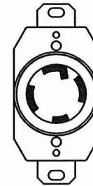
NEMA: L14-30R 125/250V-30A
