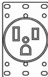
NEMA: 5-50R 125V-50A
