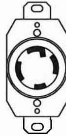
NEMA: L14-30R 125/250V-30A
