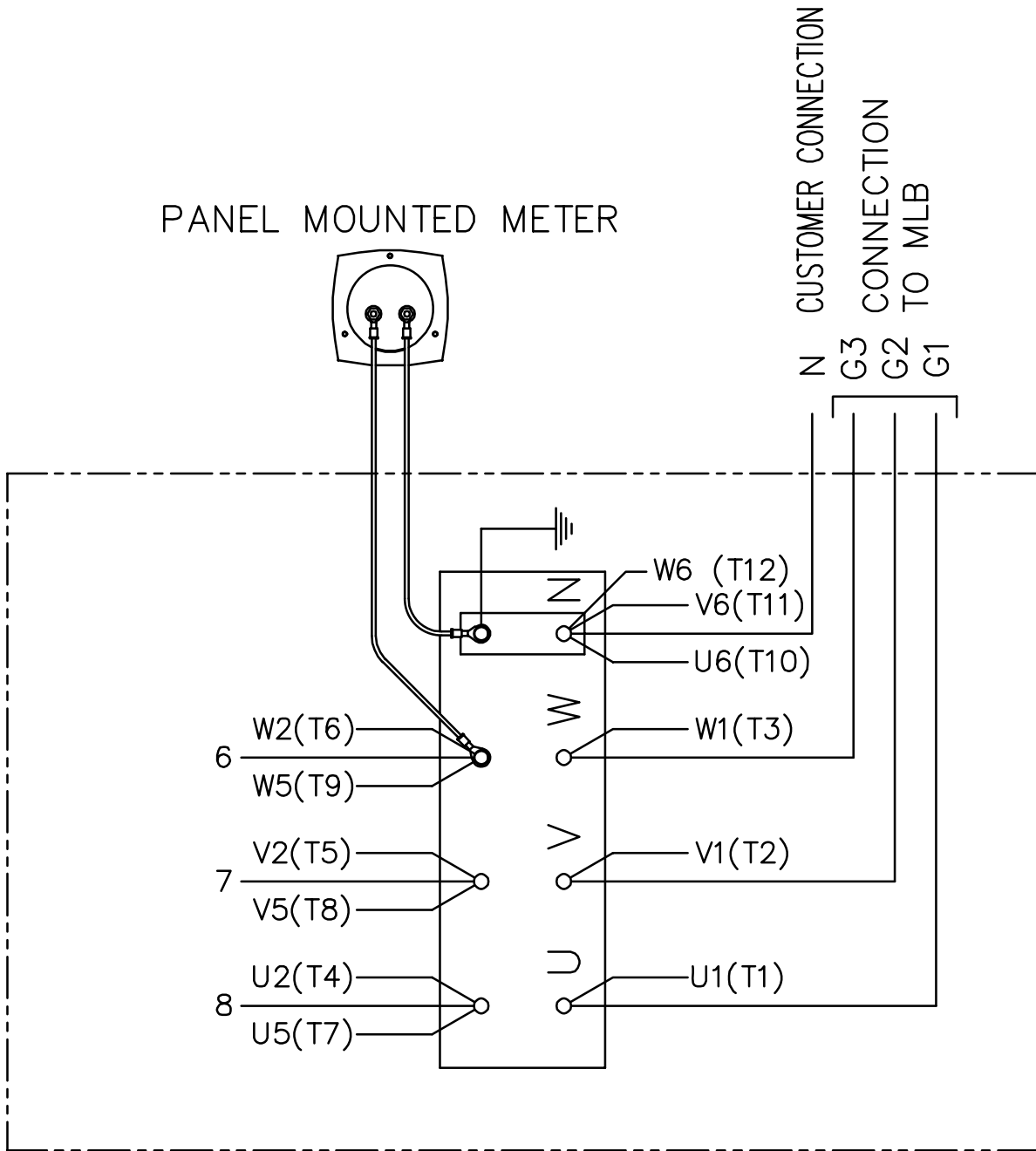
CONNECTION DIAGRAM (3 \phi SERIES WYE; 277/480)
